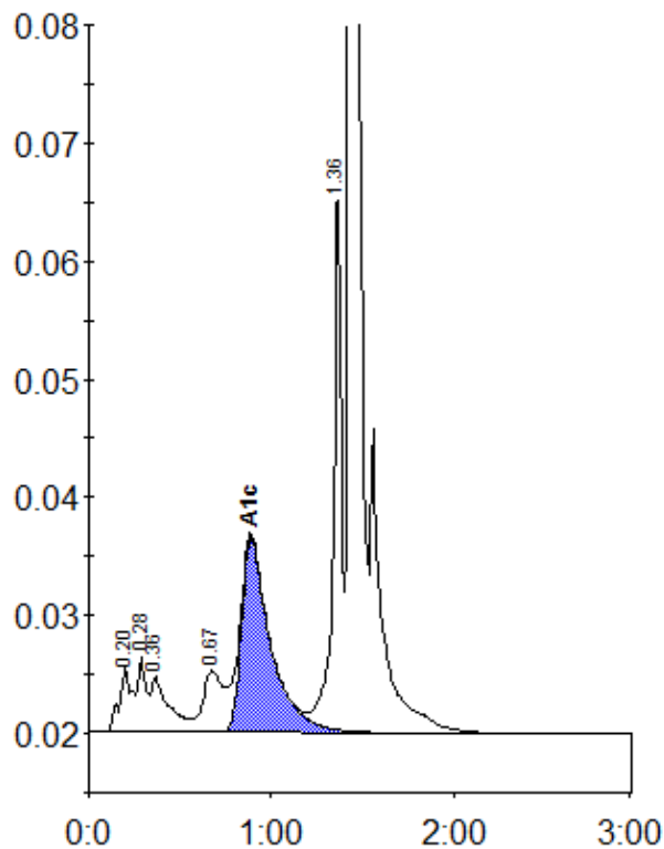
Peak table - ID: 10607057
